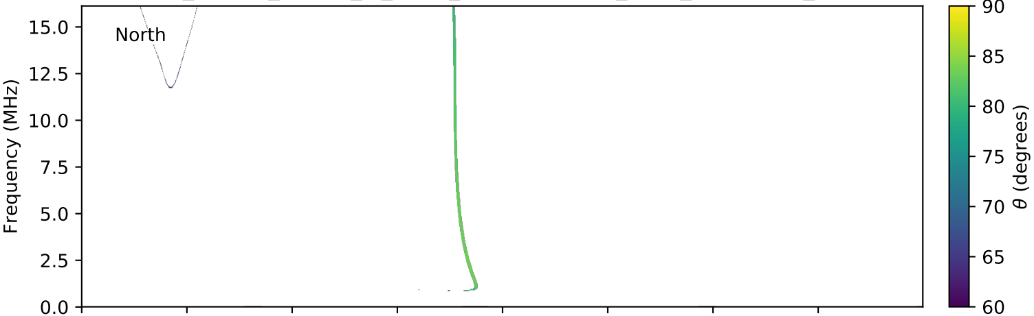
expres_cassini_jupiter_io_isaac_lossc-wid1deg_3kev_20010317_v01.cdf
