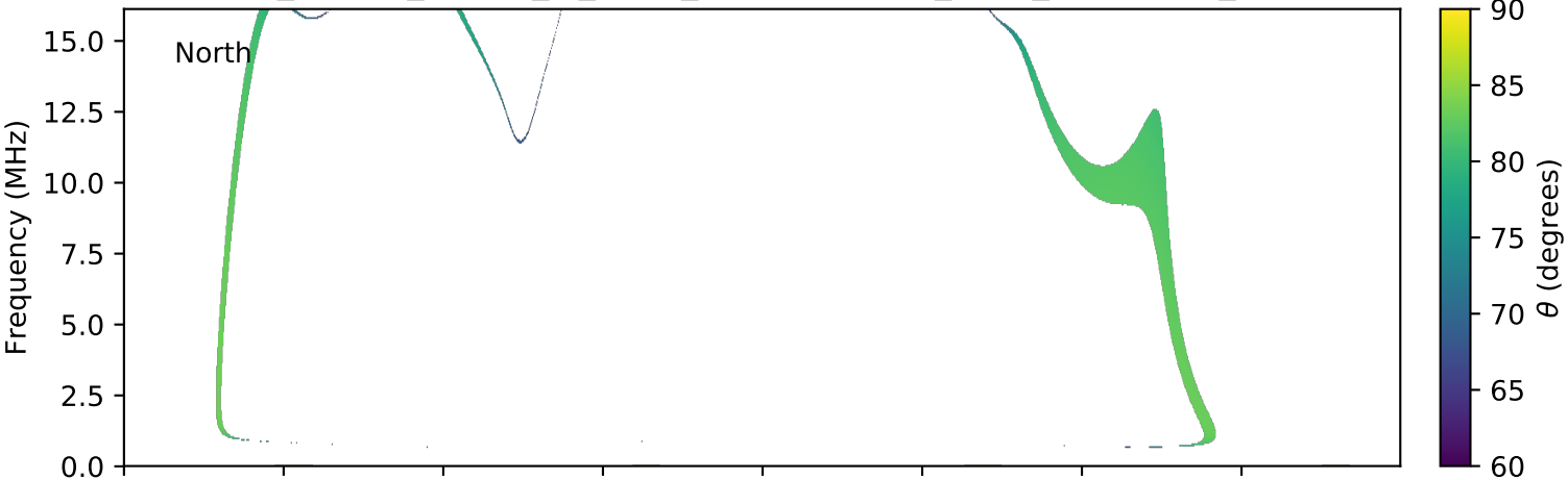
expres_cassini_jupiter_io_isaac_lossc-wid1deg_3kev_20010306_v01.cdf
