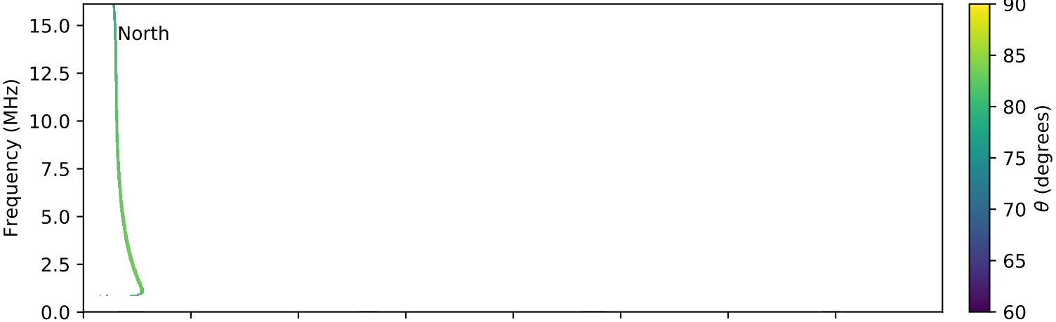
expres_cassini_jupiter_io_isaac_lossc-wid1deg_3kev_20010305_v01.cdf
