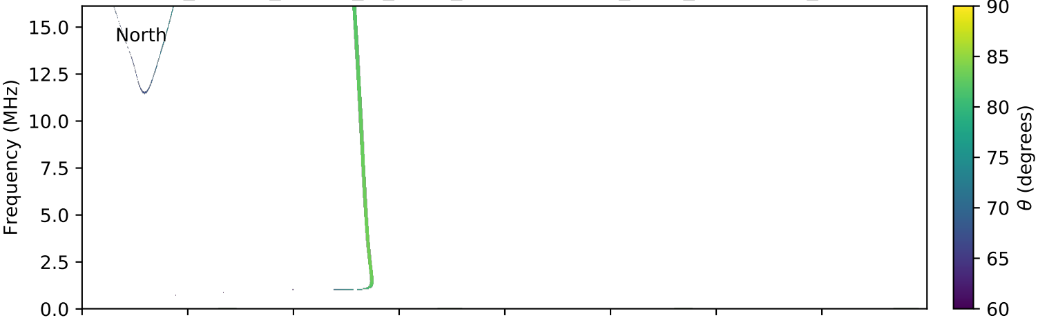
expres_cassini_jupiter_io_isaac_lossc-wid1deg_3kev_20010303_v01.cdf
