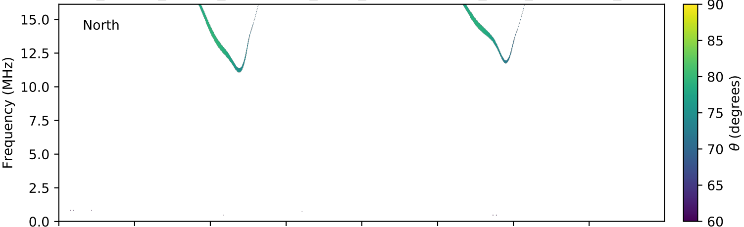
expres_cassini_jupiter_ganymede_isaac_lossc-wid1deg_3kev_20010330_v01.cdf
