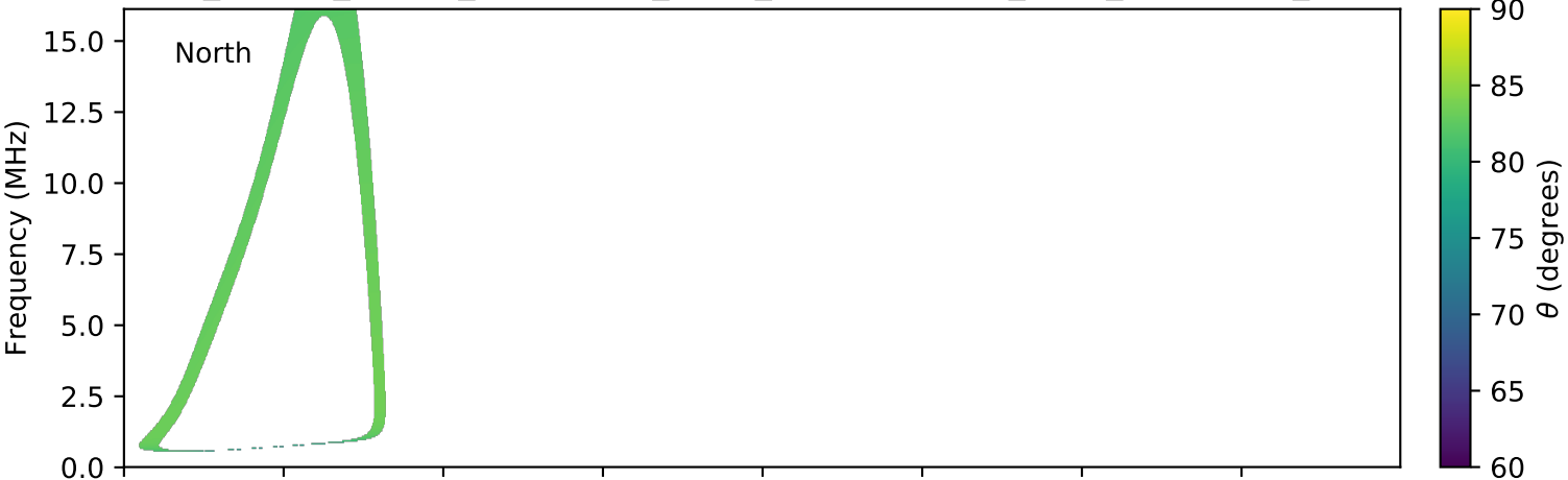
expres_cassini_jupiter_ganymede_isaac_lossc-wid1deg_3kev_20010325_v01.cdf
