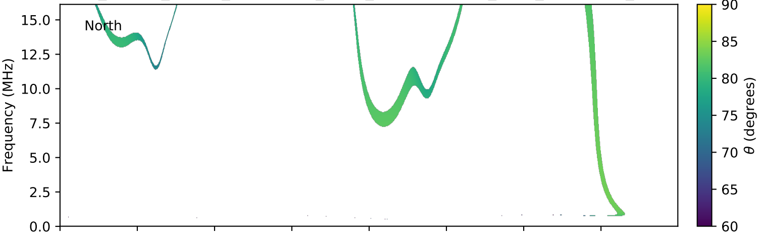
expres_cassini_jupiter_ganymede_isaac_lossc-wid1deg_3kev_20010324_v01.cdf
