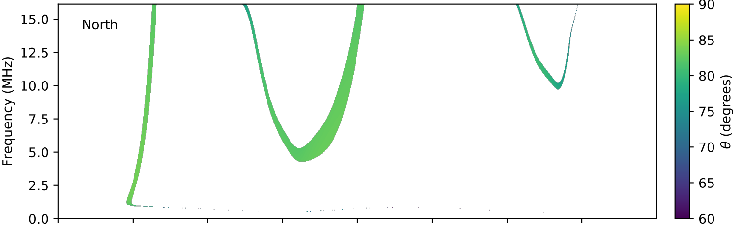
expres_cassini_jupiter_ganymede_isaac_lossc-wid1deg_3kev_20010322_v01.cdf
