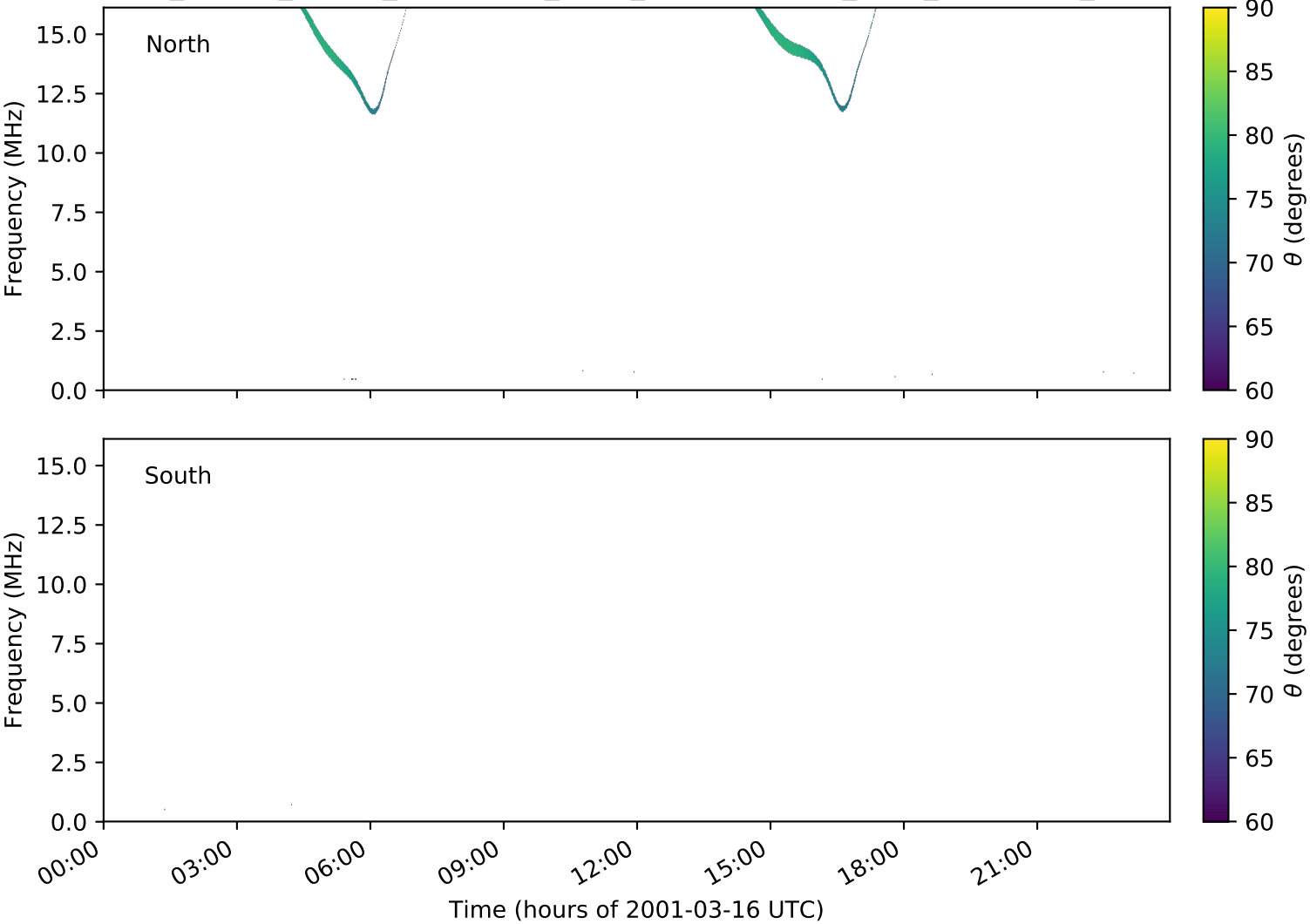
expres_cassini_jupiter_ganymede_isaac_lossc-wid1deg_3kev_20010316_v01.cdf
