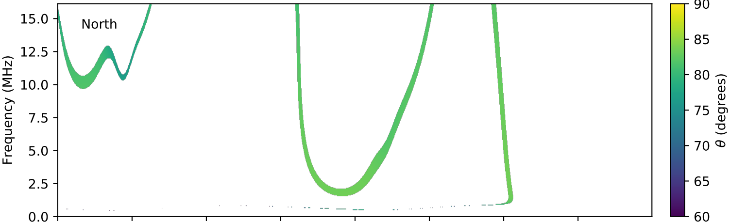
expres_cassini_jupiter_ganymede_isaac_lossc-wid1deg_3kev_20010310_v01.cdf
