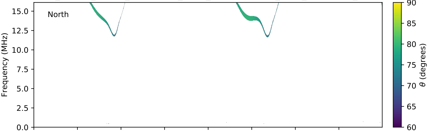
expres_cassini_jupiter_ganymede_isaac_lossc-wid1deg_3kev_20010309_v01.cdf
