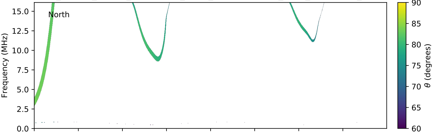
expres_cassini_jupiter_ganymede_isaac_lossc-wid1deg_3kev_20010308_v01.cdf
