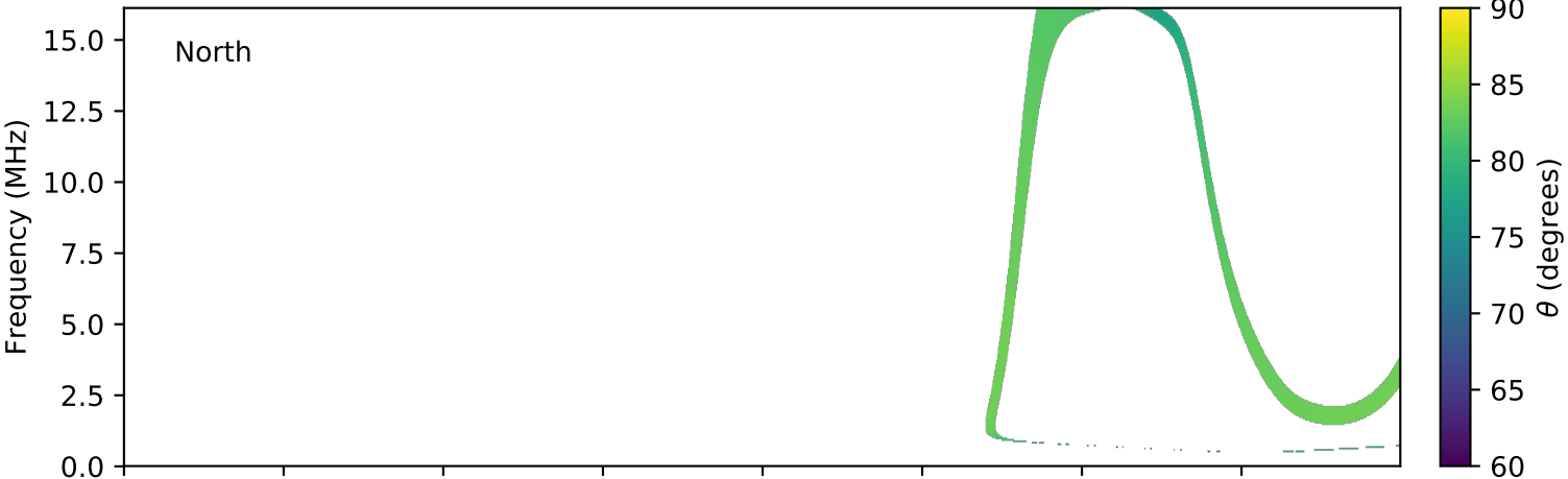
expres_cassini_jupiter_ganymede_isaac_lossc-wid1deg_3kev_20010307_v01.cdf
