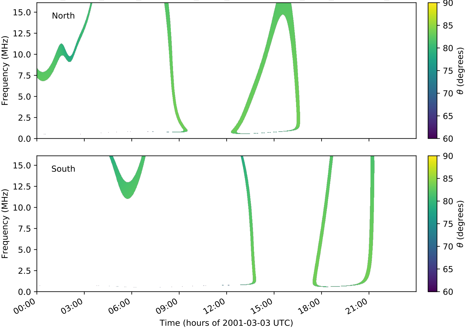
expres_cassini_jupiter_ganymede_isaac_lossc-wid1deg_3kev_20010303_v01.cdf
