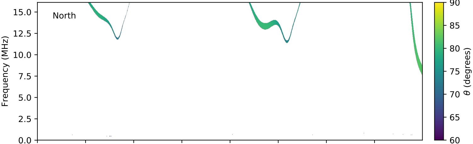
expres_cassini_jupiter_ganymede_isaac_lossc-wid1deg_3kev_20010302_v01.cdf
