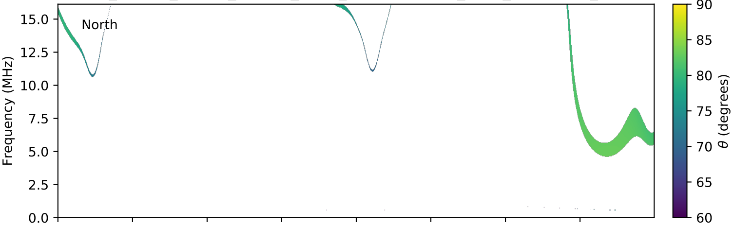
expres_cassini_jupiter_europa_isaac_lossc-wid1deg_3kev_20010329_v01.cdf
