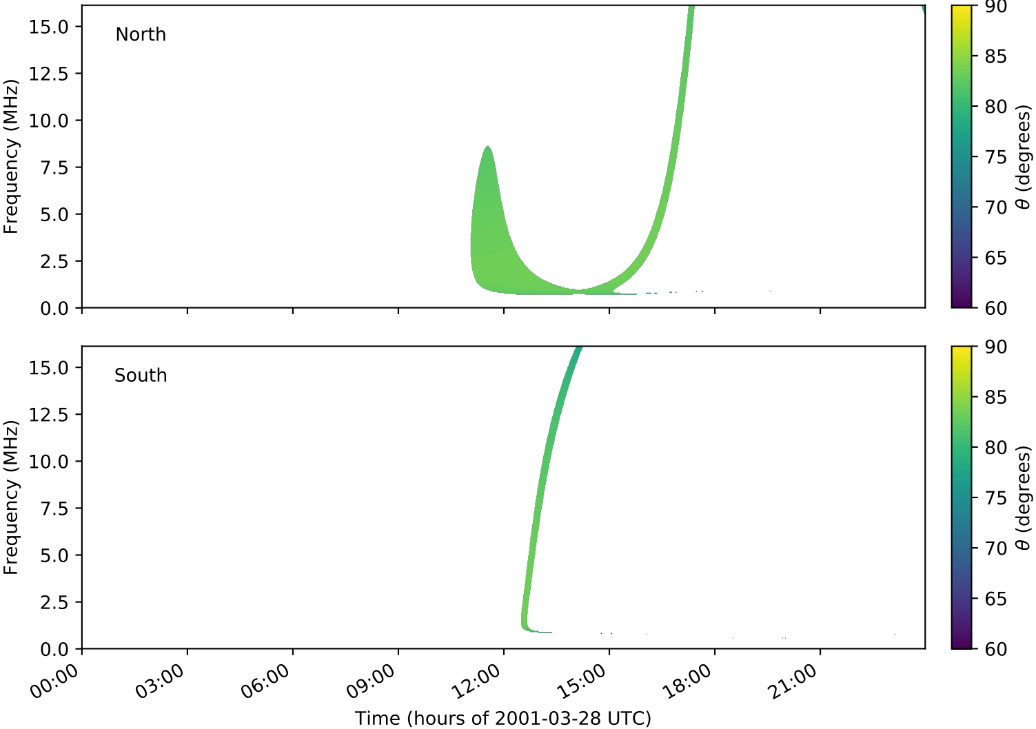
expres_cassini_jupiter_europa_isaac_lossc-wid1deg_3kev_20010328_v01.cdf
