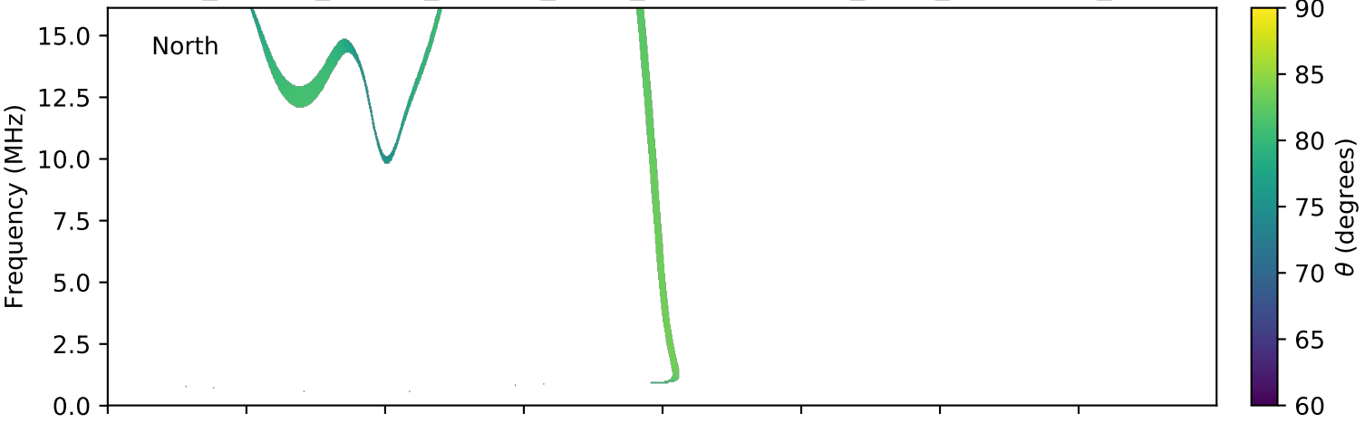
expres_cassini_jupiter_europa_isaac_lossc-wid1deg_3kev_20010326_v01.cdf
