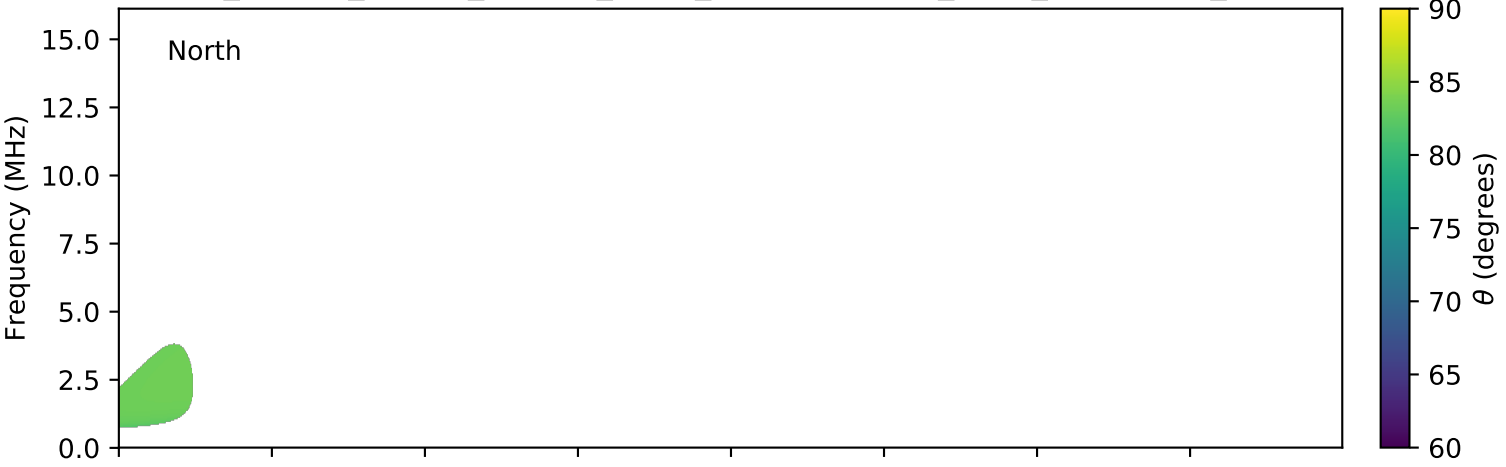
expres_cassini_jupiter_europa_isaac_lossc-wid1deg_3kev_20010323_v01.cdf
