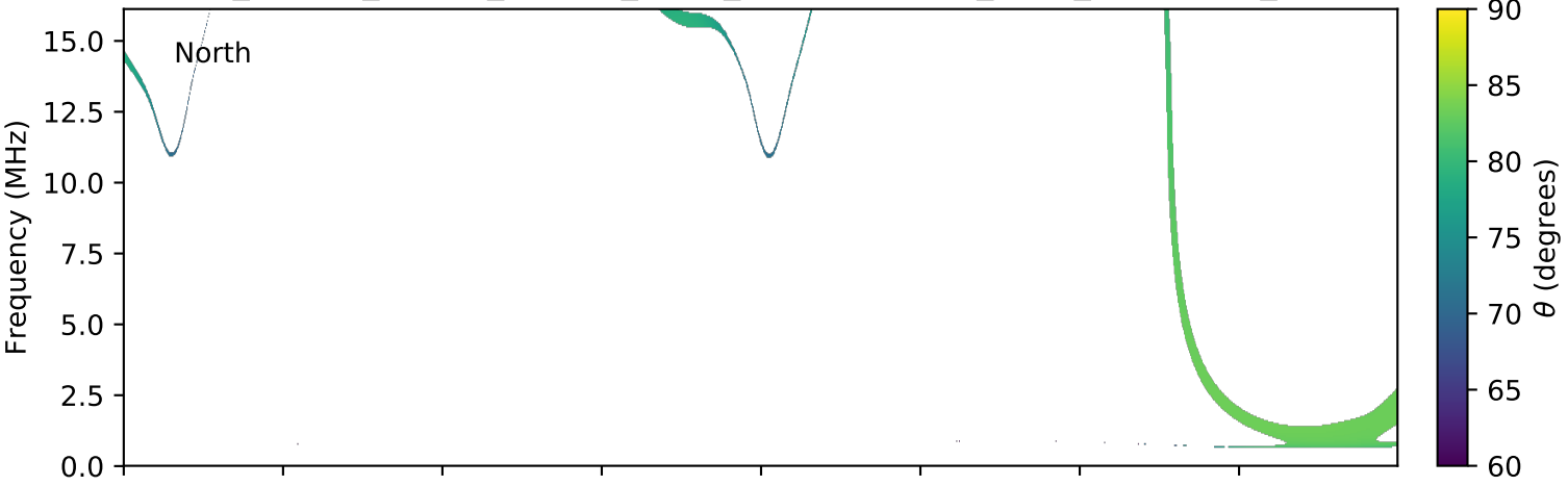
expres_cassini_jupiter_europa_isaac_lossc-wid1deg_3kev_20010322_v01.cdf
