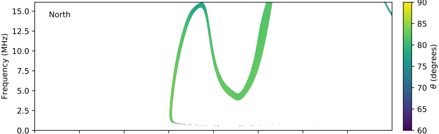
expres_cassini_jupiter_europa_isaac_lossc-wid1deg_3kev_20010321_v01.cdf
