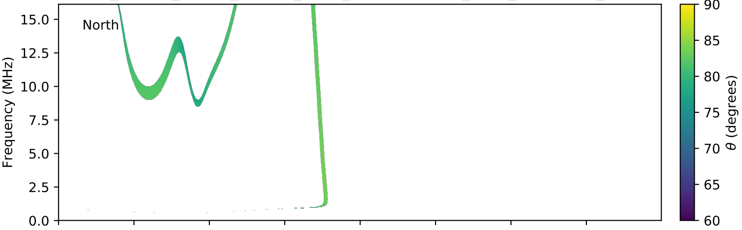
expres_cassini_jupiter_europa_isaac_lossc-wid1deg_3kev_20010319_v01.cdf
