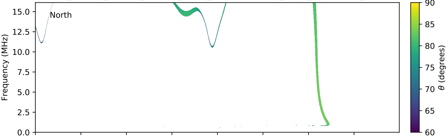
expres_cassini_jupiter_europa_isaac_lossc-wid1deg_3kev_20010315_v01.cdf
