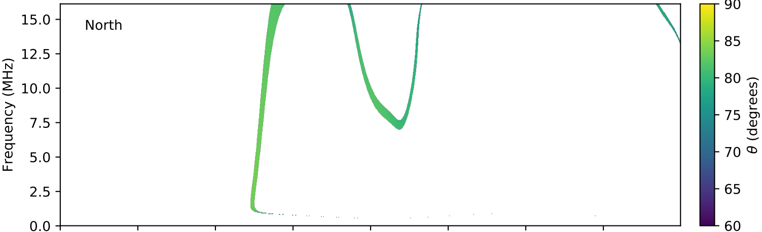
expres_cassini_jupiter_europa_isaac_lossc-wid1deg_3kev_20010314_v01.cdf
