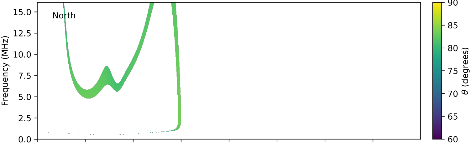
expres_cassini_jupiter_europa_isaac_lossc-wid1deg_3kev_20010312_v01.cdf
