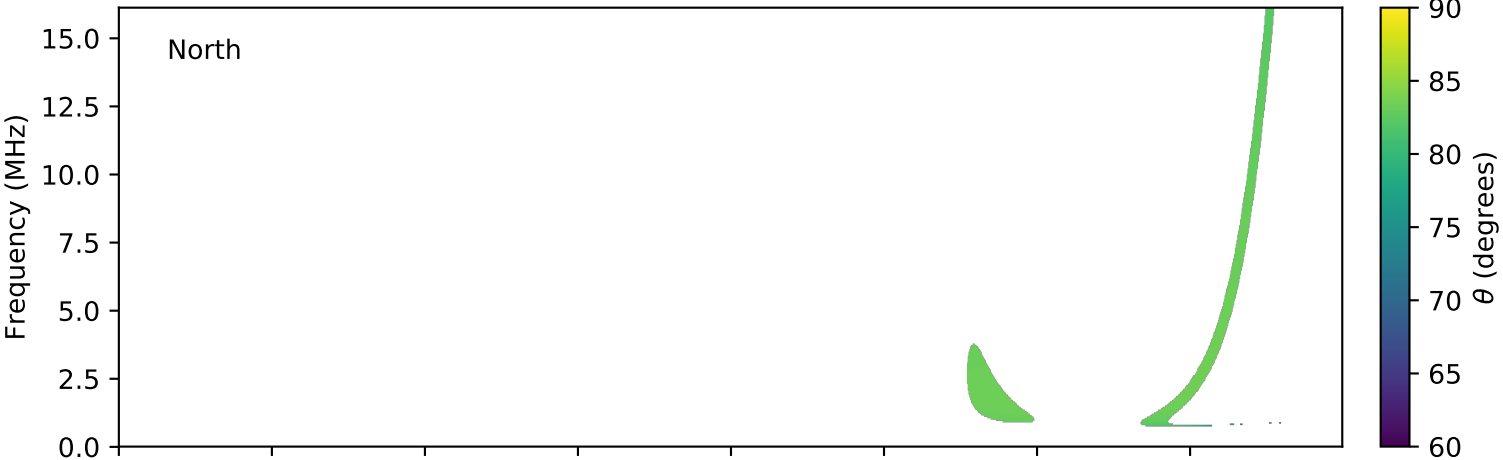
expres_cassini_jupiter_europa_isaac_lossc-wid1deg_3kev_20010310_v01.cdf
