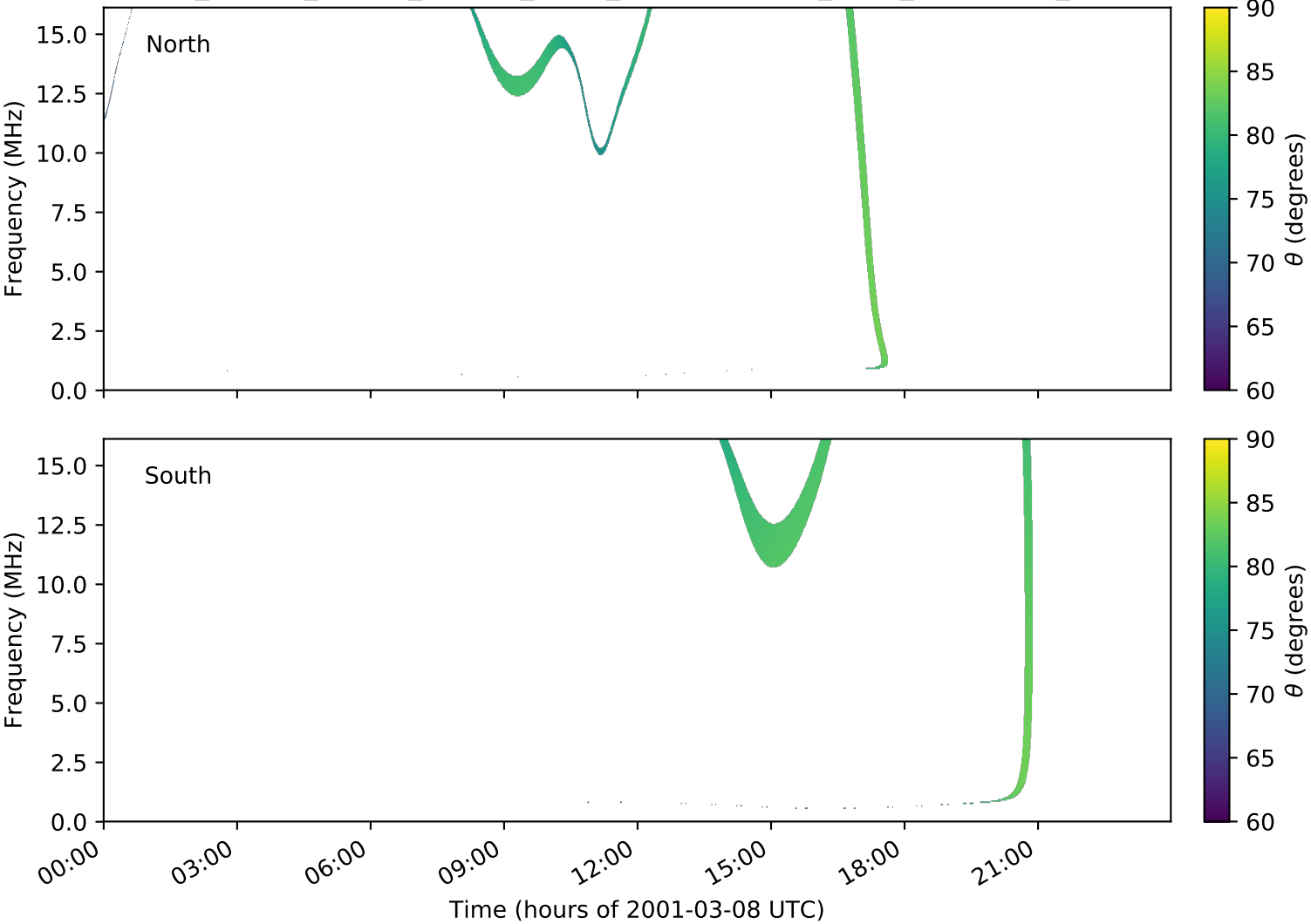
expres_cassini_jupiter_europa_isaac_lossc-wid1deg_3kev_20010308_v01.cdf
