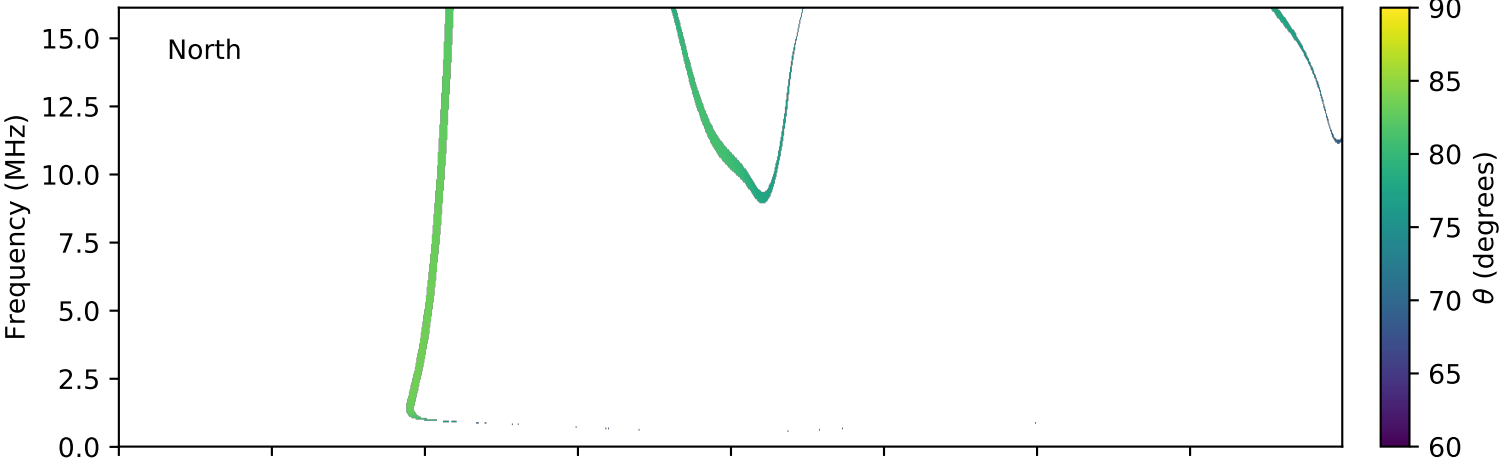
expres_cassini_jupiter_europa_isaac_lossc-wid1deg_3kev_20010307_v01.cdf
