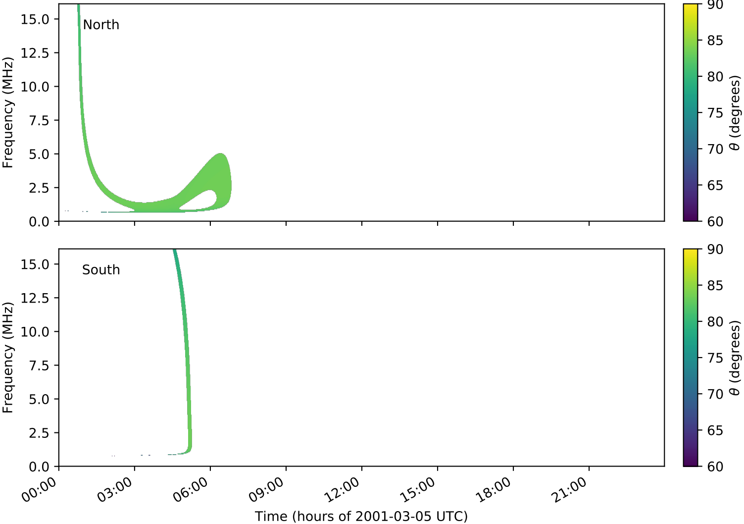
expres_cassini_jupiter_europa_isaac_lossc-wid1deg_3kev_20010305_v01.cdf
