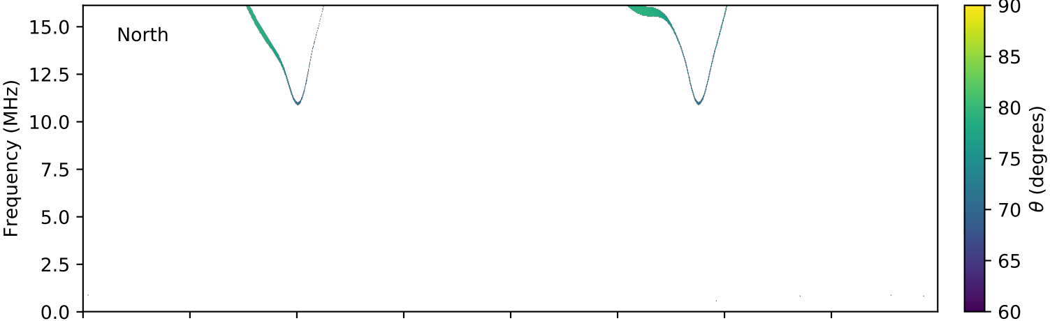
expres_cassini_jupiter_europa_isaac_lossc-wid1deg_3kev_20010304_v01.cdf
