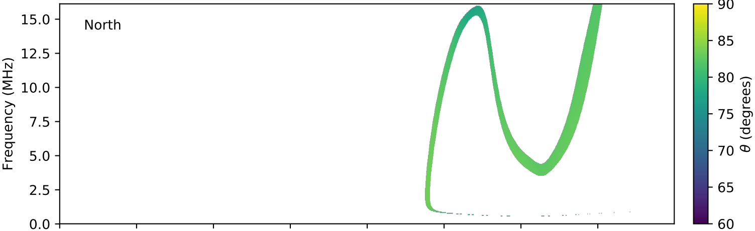
expres_cassini_jupiter_europa_isaac_lossc-wid1deg_3kev_20010303_v01.cdf
