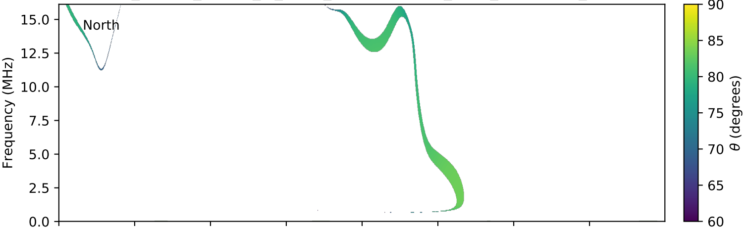
expres_cassini_jupiter_io_isaac_lossc-wid1deg_3kev_20010128_v01.cdf
