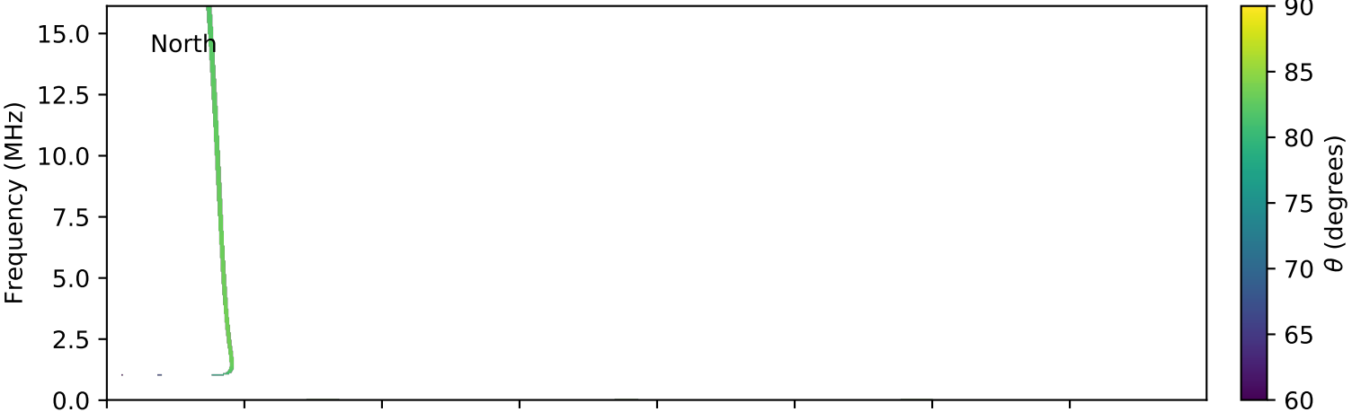
expres_cassini_jupiter_io_isaac_lossc-wid1deg_3kev_20010125_v01.cdf
