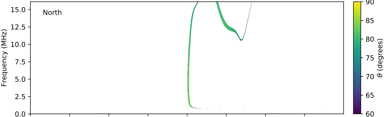
expres_cassini_jupiter_io_isaac_lossc-wid1deg_3kev_20010122_v01.cdf
