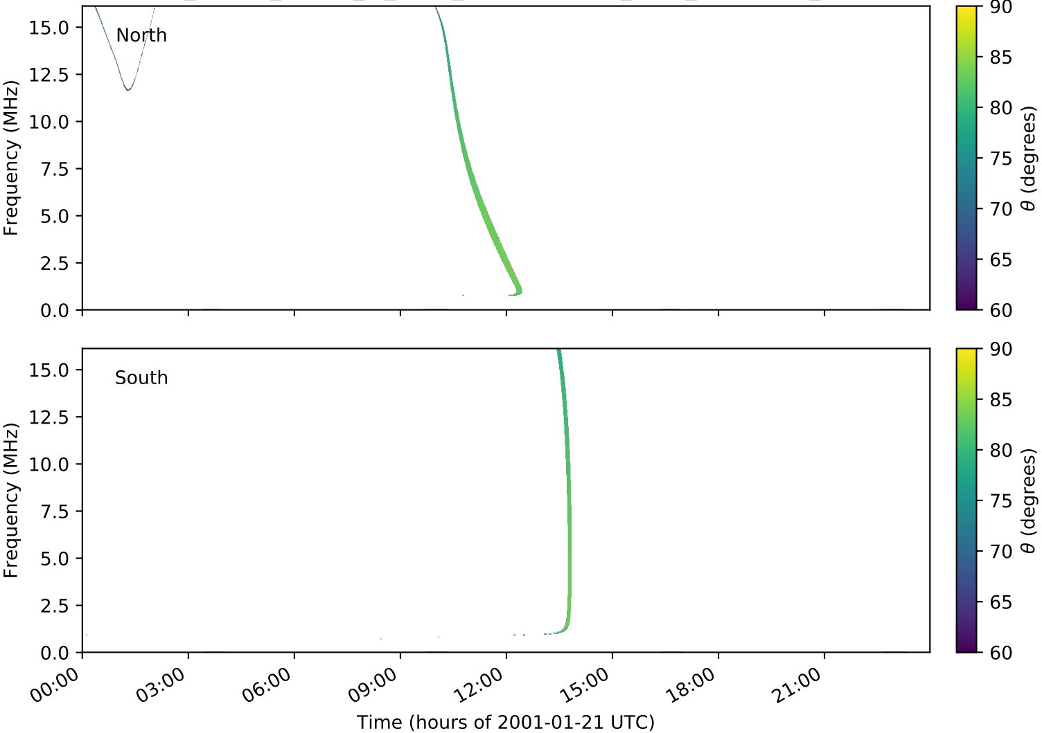
expres_cassini_jupiter_io_isaac_lossc-wid1deg_3kev_20010121_v01.cdf
