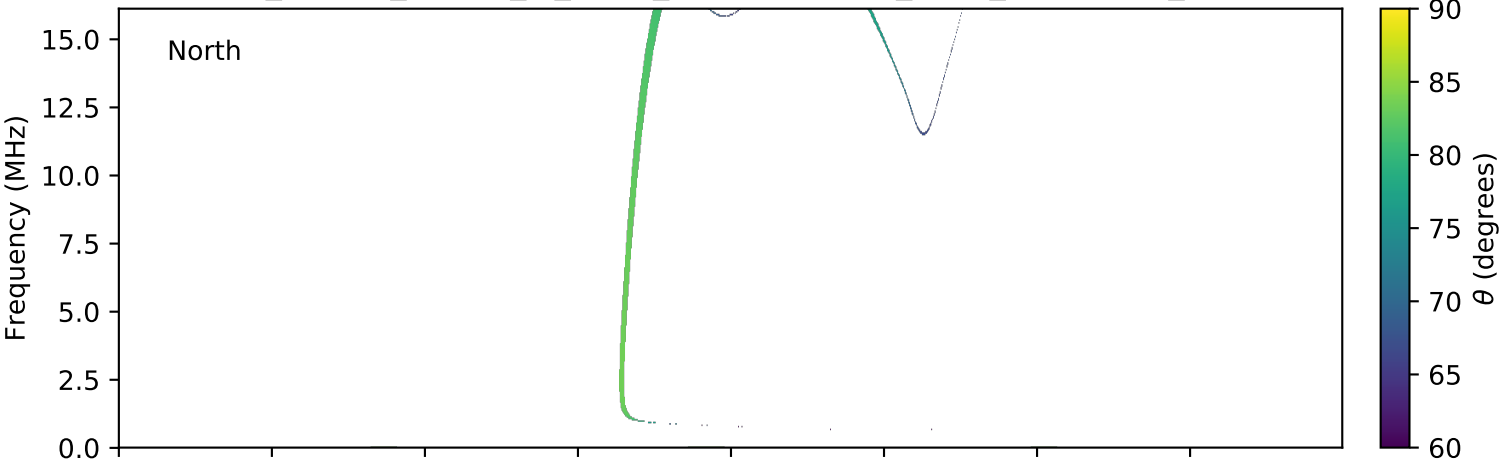
expres_cassini_jupiter_io_isaac_lossc-wid1deg_3kev_20010115_v01.cdf
