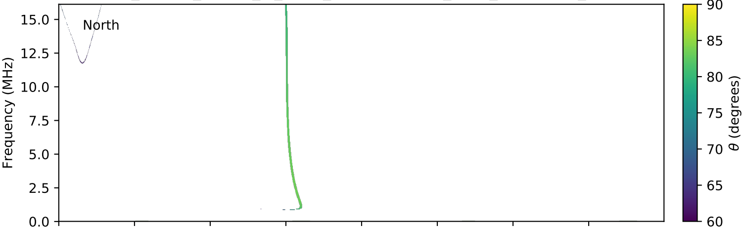
expres_cassini_jupiter_io_isaac_lossc-wid1deg_3kev_20010114_v01.cdf
