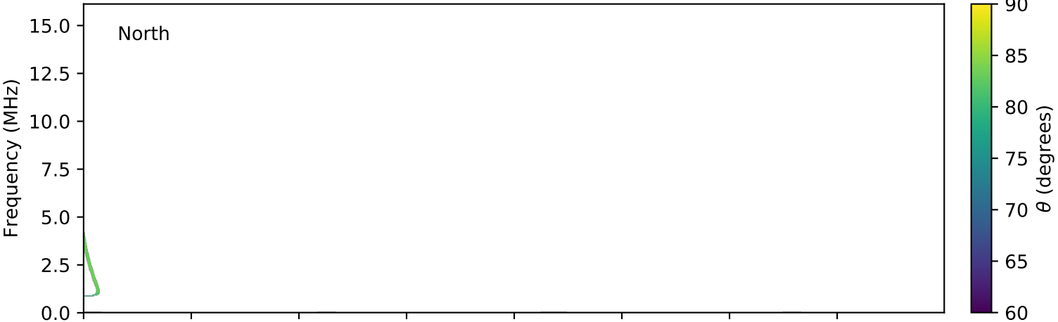
expres_cassini_jupiter_io_isaac_lossc-wid1deg_3kev_20010109_v01.cdf
