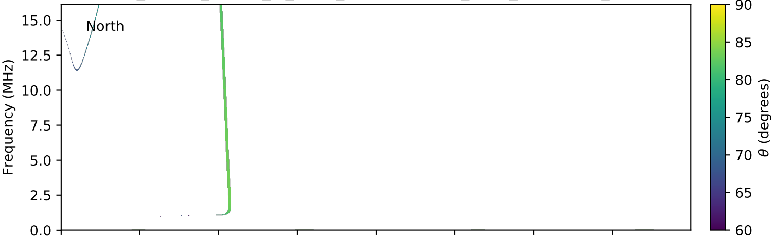
expres_cassini_jupiter_io_isaac_lossc-wid1deg_3kev_20010107_v01.cdf
