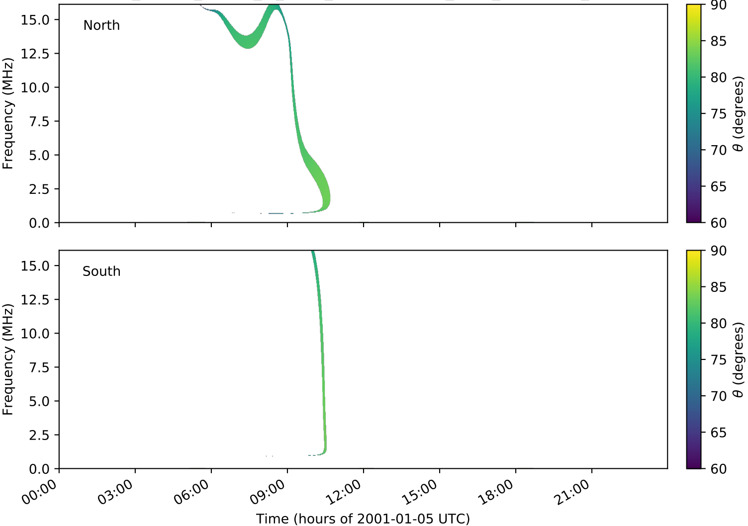
expres_cassini_jupiter_io_isaac_lossc-wid1deg_3kev_20010105_v01.cdf
