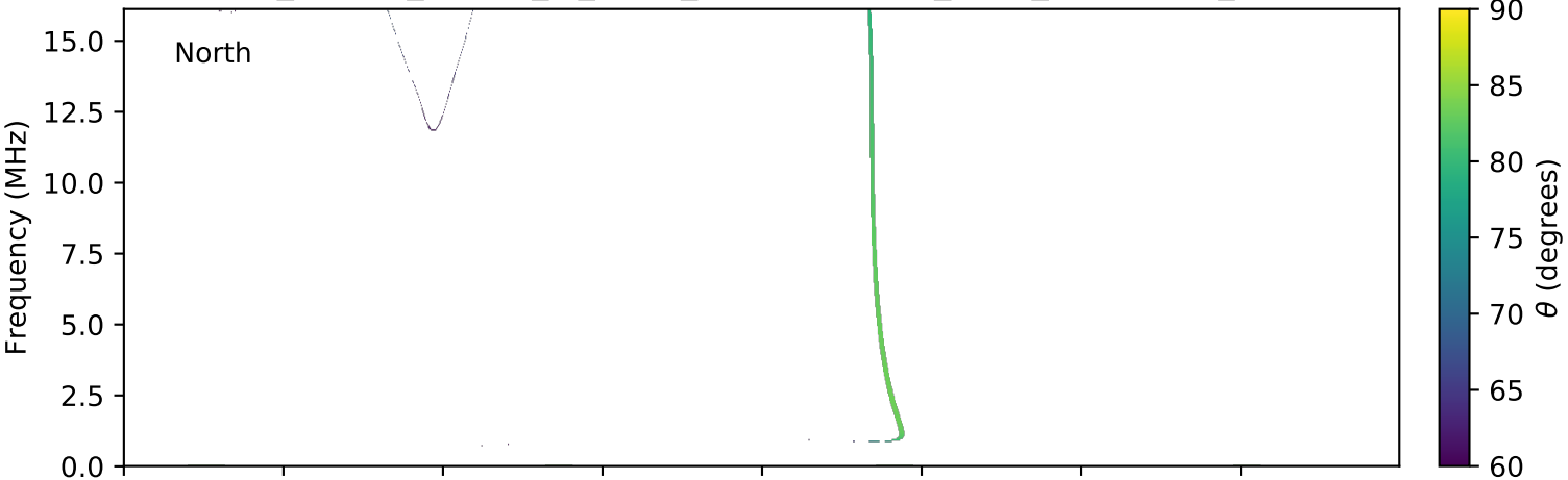
expres_cassini_jupiter_io_isaac_lossc-wid1deg_3kev_20010103_v01.cdf
