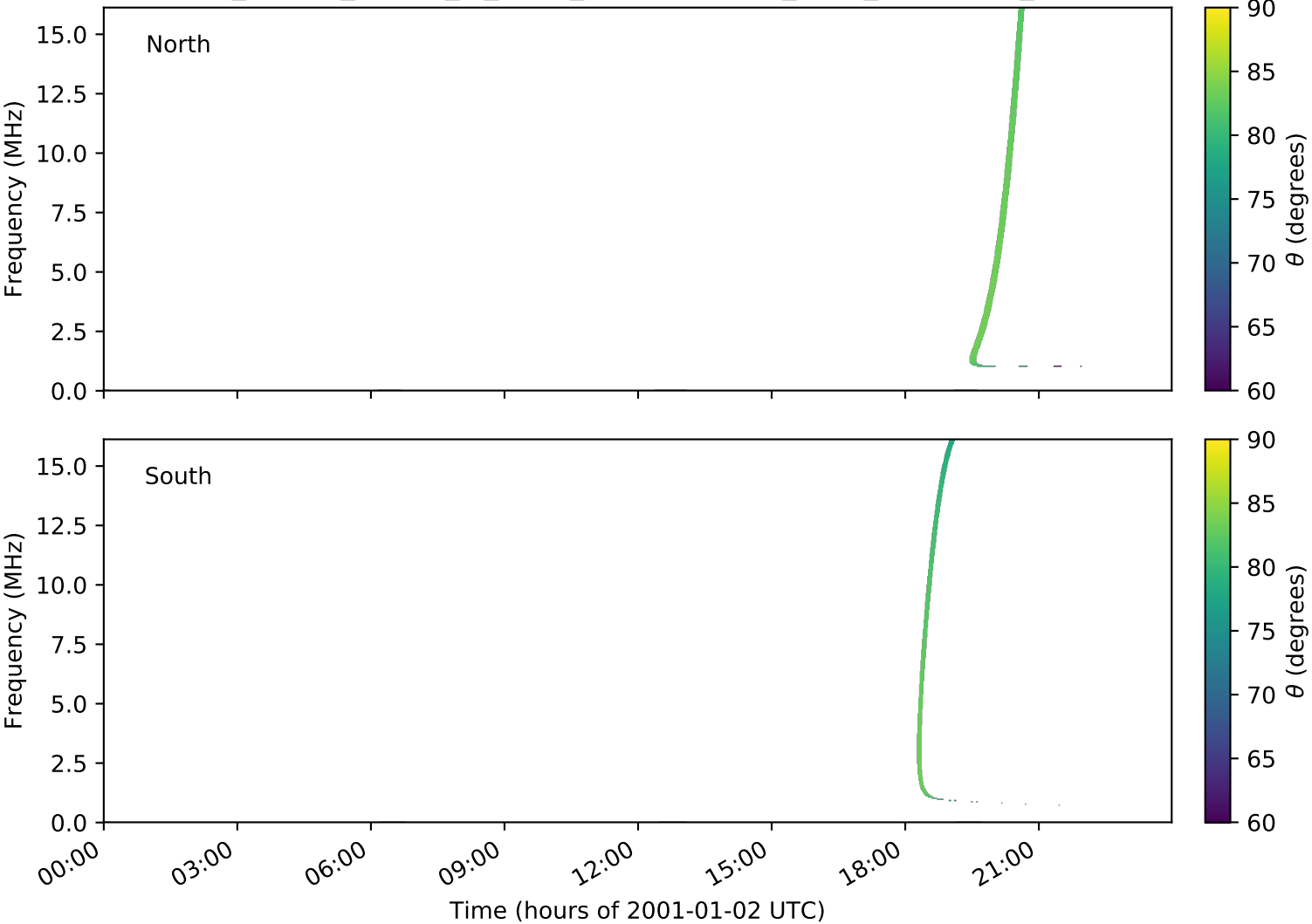
expres_cassini_jupiter_io_isaac_lossc-wid1deg_3kev_20010102_v01.cdf
