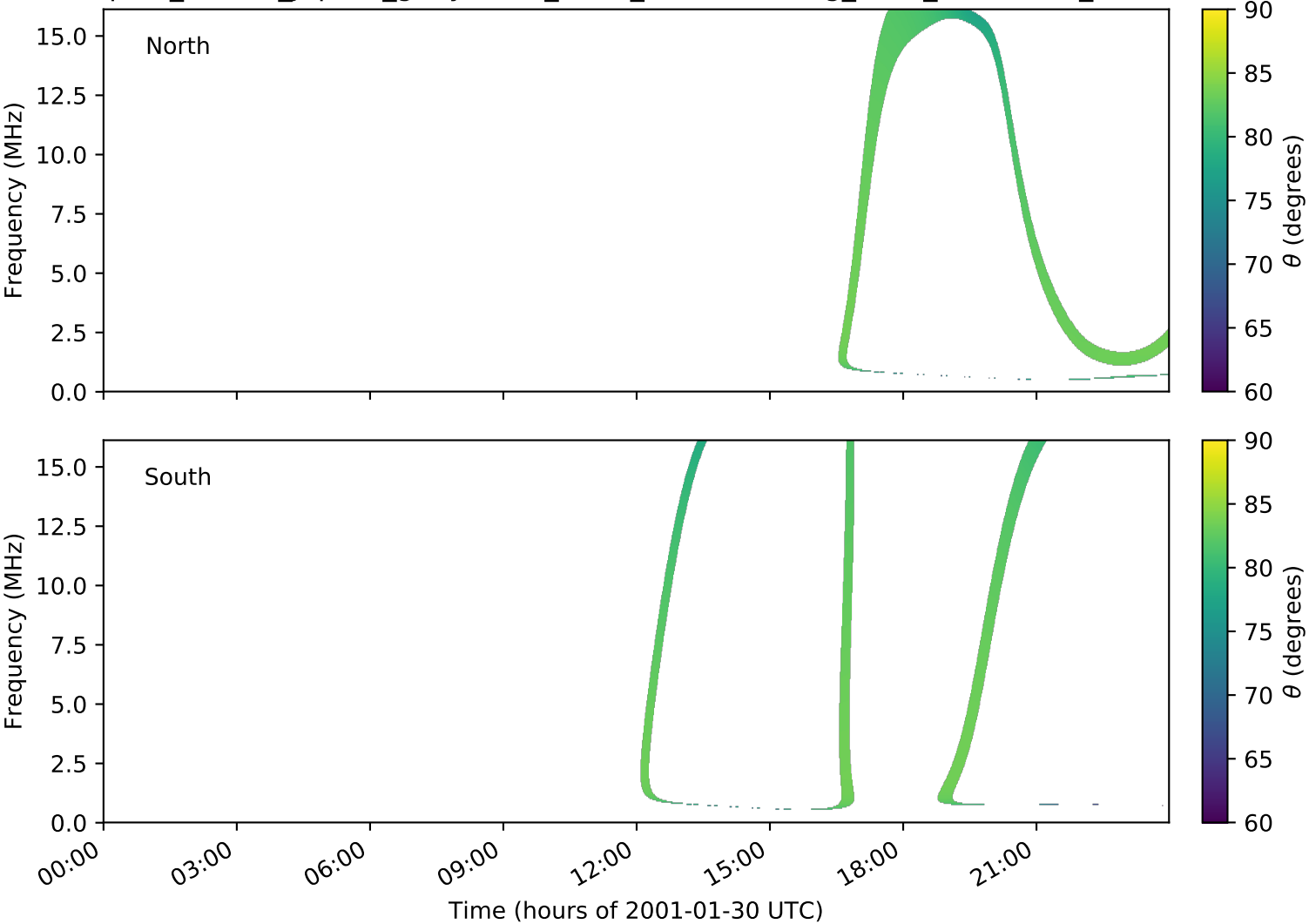
expres_cassini_jupiter_ganymede_isaac_lossc-wid1deg_3kev_20010130_v01.cdf
