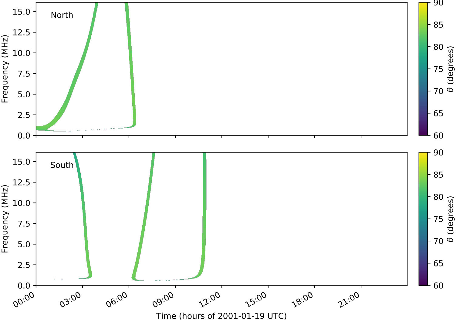
expres_cassini_jupiter_ganymede_isaac_lossc-wid1deg_3kev_20010119_v01.cdf
