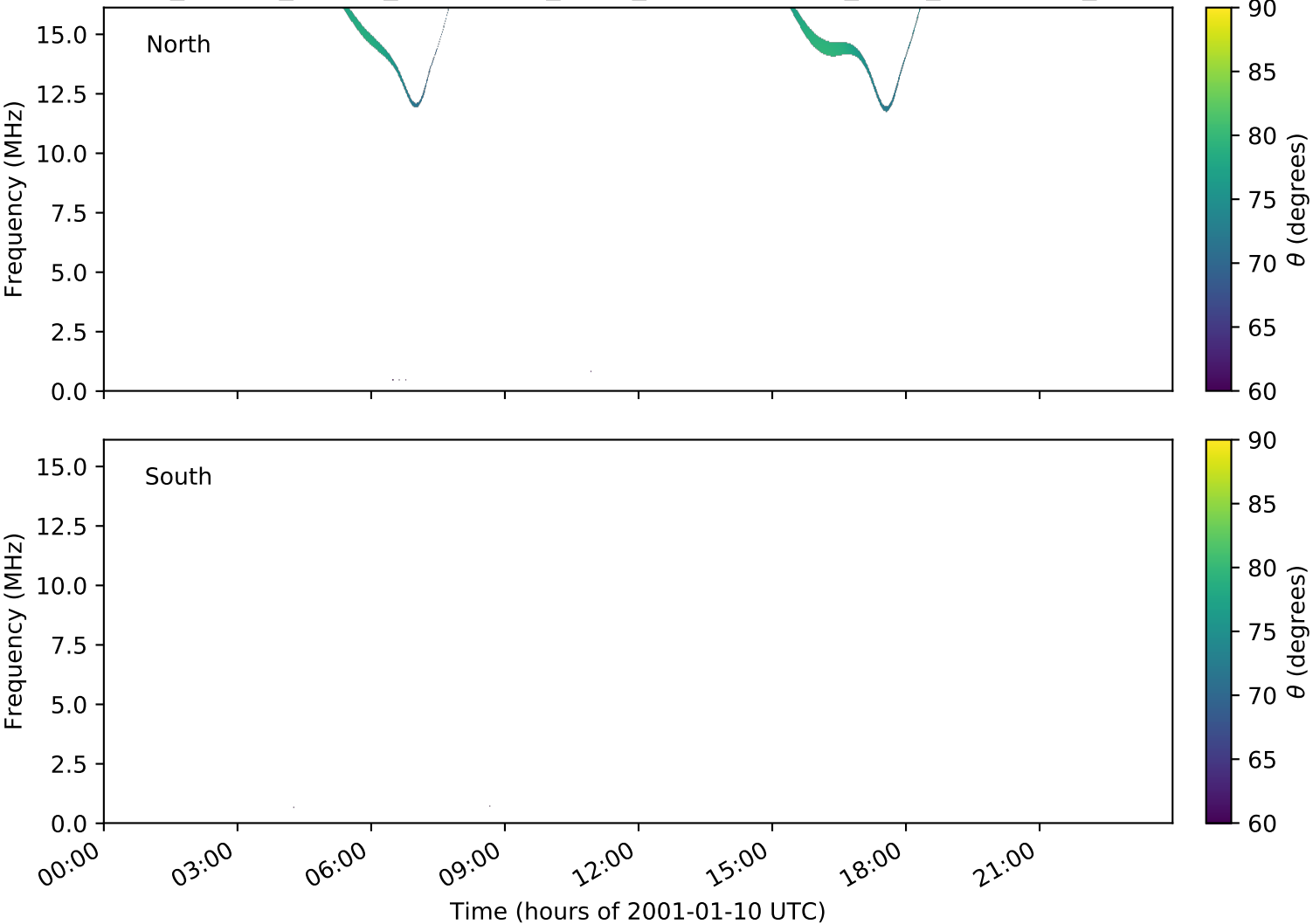
expres_cassini_jupiter_ganymede_isaac_lossc-wid1deg_3kev_20010110_v01.cdf
