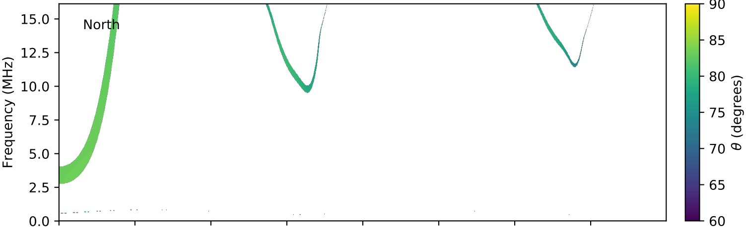
expres_cassini_jupiter_ganymede_isaac_lossc-wid1deg_3kev_20010109_v01.cdf
