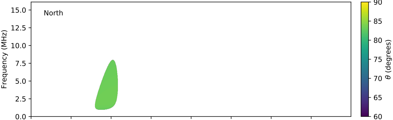
expres_cassini_jupiter_ganymede_isaac_lossc-wid1deg_3kev_20010104_v01.cdf
