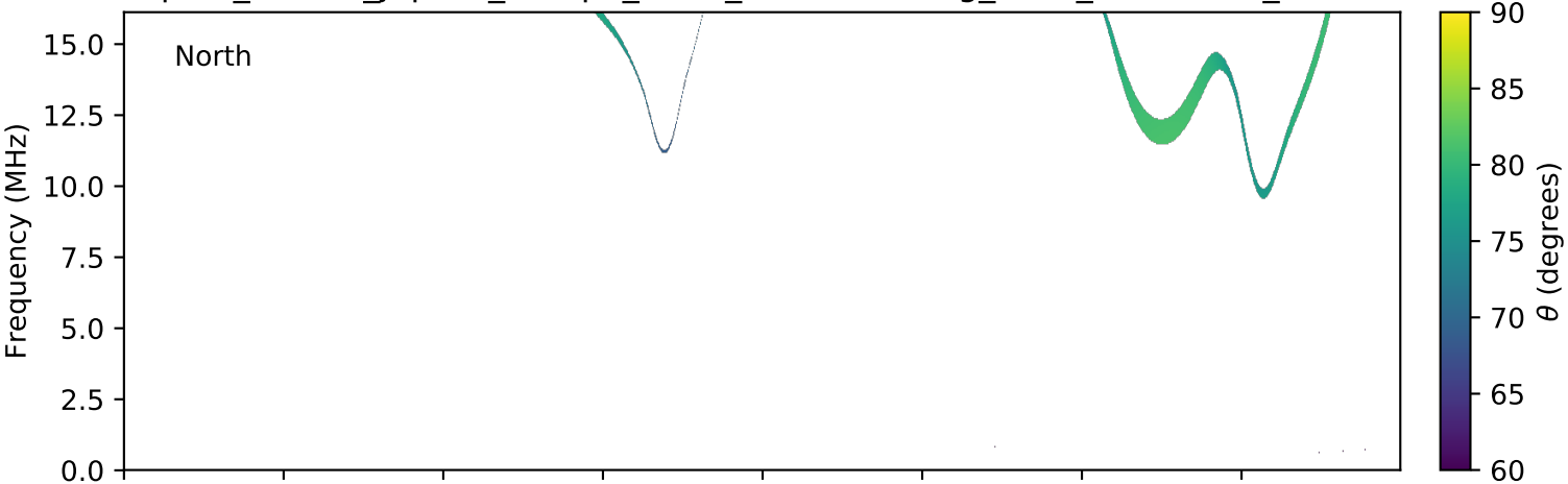
expres_cassini_jupiter_europa_isaac_lossc-wid1deg_3kev_20010131_v01.cdf
