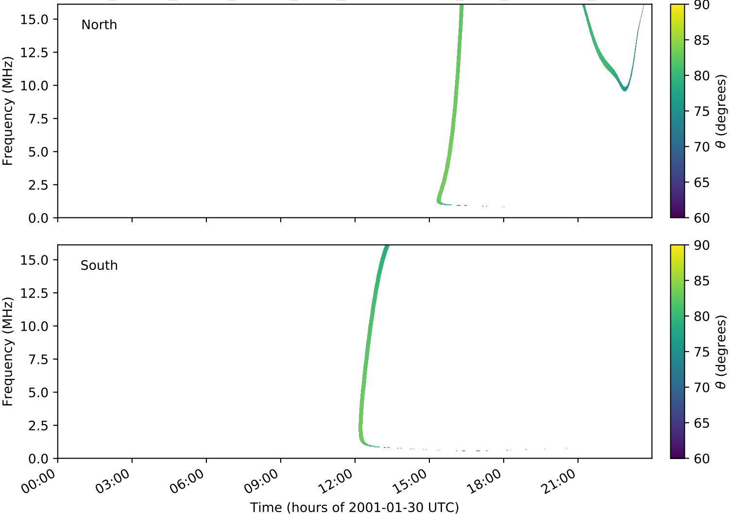
expres_cassini_jupiter_europa_isaac_lossc-wid1deg_3kev_20010130_v01.cdf
