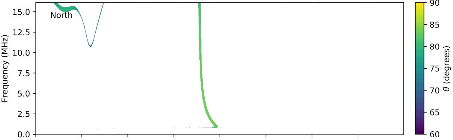
expres_cassini_jupiter_europa_isaac_lossc-wid1deg_3kev_20010128_v01.cdf
